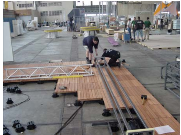
EXHIBITION FLOORING - BUZON PEDESTAL & TILE COMBINATION
